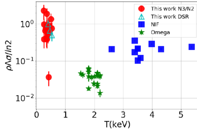
Figure 4: (color online) \rho\Lambda\sigma/\ln 2 obtained from eq.(4) vs T from eq.(1). Omega and NIF data are derived from the experiments[25], using the Down Scatter Ratio[23, 21]. Our results using the DSR method ( N_4/N_3 ) are given by the open triangle symbols in good agreement with the N_3/N_2 ratios.
