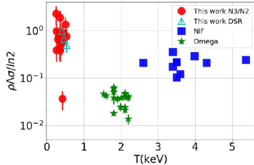
Figure 4: (color online) \rho \Lambda \sigma / \ln 2 obtained from eq.(4) vs T from eq.(1). Omega and NIF data are derived from the experiments[25], using the Down Scatter Ratio[23, 21]. Our results using the DSR method ( N_4/N_3 ) are given by the open triangle symbols in good agreement with the N_3/N_2 ratios.
